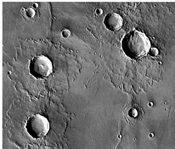
Figure 4. Impact craters in Lunae Planum. As is typical of Martian craters, material ejected during each impact is arrayed in lobes outlined by low ridges. The pattern is very different from that around lunar impact craters — either because of the properties of the surface materials or because of the presence of an atmosphere. Although these craters are probably billions of years old they are almost perfectly preserved, implying extremely low erosion rates. The largest crater is 20 km across.
