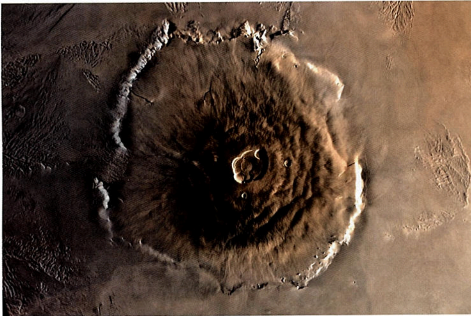
Figure 9. The huge shield volcano Olympus Mons covers an area the size of Arizona. Its peak is up to 24 km above the surrounding Tharsis plateau. At the volcano's summit is a conspicuous caldera, a complex nest of craters 80 km across. A caldera forms when magma rising toward the surface stalls and fills a chamber beneath the summit. Once the magma finally erupts, the chamber collapses, which enlarges the caldera. Long before spacecraft discovered its true nature, Olympus Mons and the clouds that frequently attend it were recognized by telescopic observers as a bright spot on Mars named Nix Olympica (Snows of Olympus).
