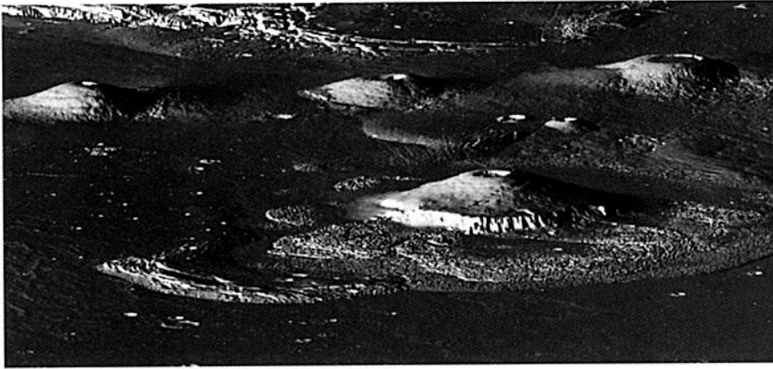
Figure 8. A topographic representation looking southeast across the Tharsis plateau, with vertical relief exaggerated three times. Olympus Mons (foreground) is 550 km across and 24 km (78,000 feet) high. The cliff along its base is itself 9 km (29,000 feet) high. Huge tongues of highly textured terrain, just visible in front of the cliff, were perhaps caused by a series of collapses of the volcano's outer flanks. In the distance are (left to right) Ascreaus Mons, Pavonis Mons, and Arsia Mons — all likewise huge volcanoes by terrestrial standards. Beyond them lies Valles Marineris.
