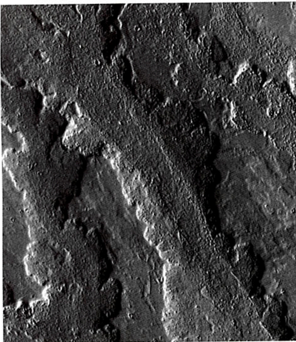
Figure 5. Most of the plains of Tharsis consist of lava flows stacked one upon another. Here a 4-km-wide flow, which erupted from the flanks of Pavonis Mons then spread over the adjacent plains, runs diagonally through the image. In the middle of the flow is a vaguely outlined channel that transported lava to the flow front. The flows resemble those seen on the flanks of large terrestrial volcanoes, but most are much larger and imply higher eruption rates. Illumination is from the left.
