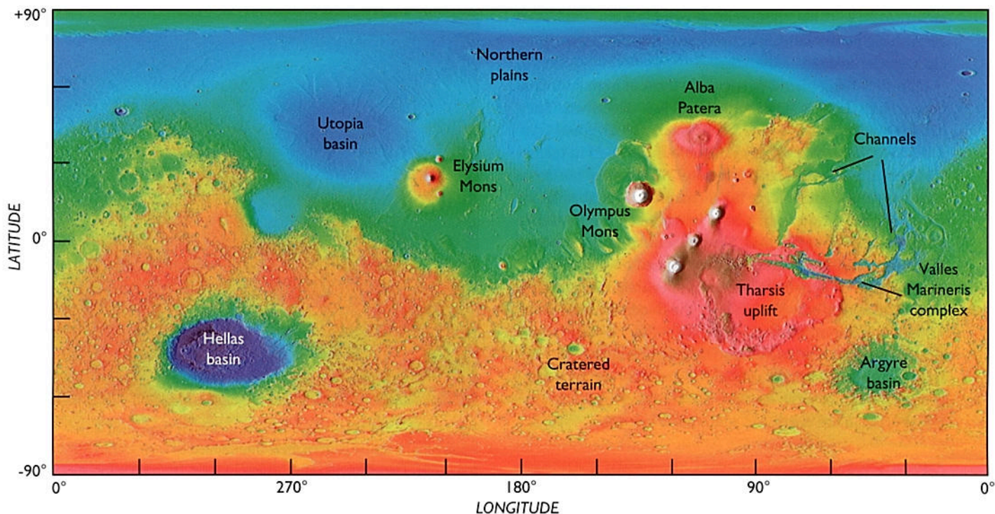
Figure 3. In this portrayal of Martian topography, reds and yellows denote high areas while blues and greens show low areas. Note the striking dichotomy between the planet's cratered highlands to the south and the low-lying sparsely cratered plains to the north. The hemisphere at right is dominated by Tharsis, a huge volcanic pile upon which sit the planet's tallest volcanoes. The vast canyons of Valles Marineris extend eastward from the center of Tharsis. The most prominent feature in the other hemisphere is Hellas, a 2,200-km-wide impact basin. Just north of the equator is the volcanic feature Elysium surrounded by plains.
