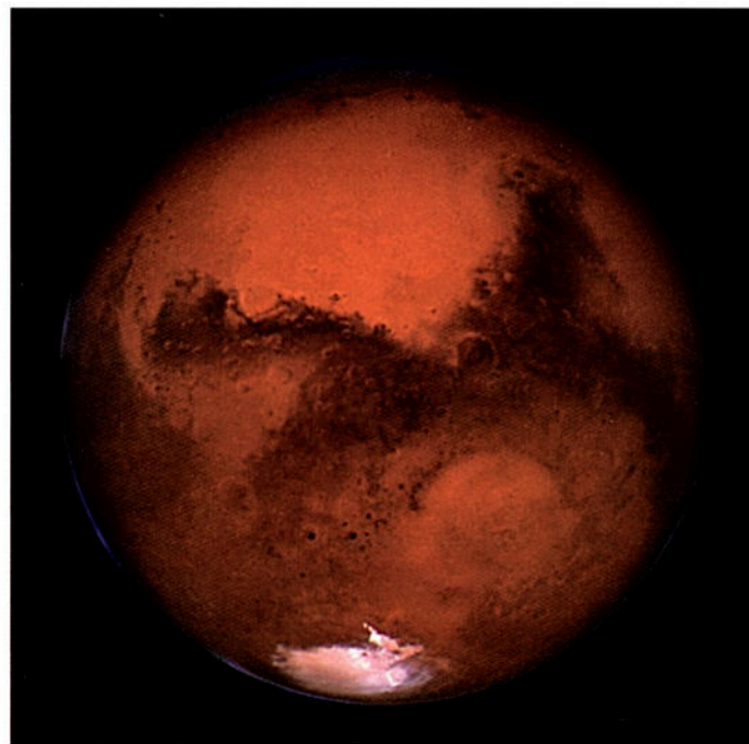
Figure 1. The Hubble Space Telescope obtained this sharp view of Mars in 2003, when the planet was slightly closer to Earth than at any time in the past 60,000 years. The bright area known as Arabia Terra (above center) is wedged between dark Sinus Meridiani at left and Syrtis Major at right. The large impact basin Hellas appears below them, to the upper right of the ice-covered south-polar cap.
