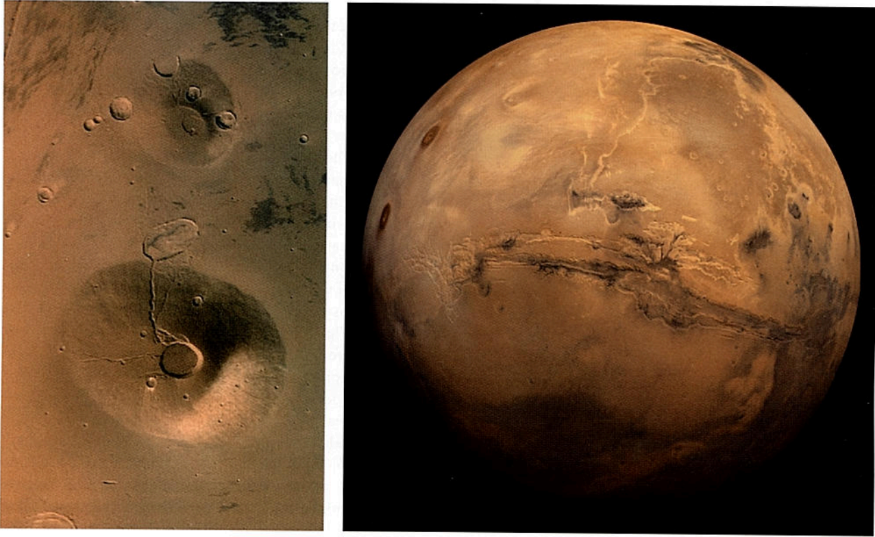
Figure 10 (left). Not all the volcanoes in Tharsis are analogs to terrestrial shield volcanoes. Ceraunius Tholus (bottom of image) has a densely channeled surface with few visible flows. The channeling suggests that the surface is composed of easily erodible material such as ash. The cause of the channels is controversial. Possibilities include erosion by water and erosion by nuées ardentes — hot, dense clouds of ash. The outer flanks of the volcano are covered by younger lava flows, and the number of impact craters superposed on the volcano flanks suggests a surface older than those of the large Tharsis shield volcanoes. We may be seeing just the summits of two old, larger shields.
